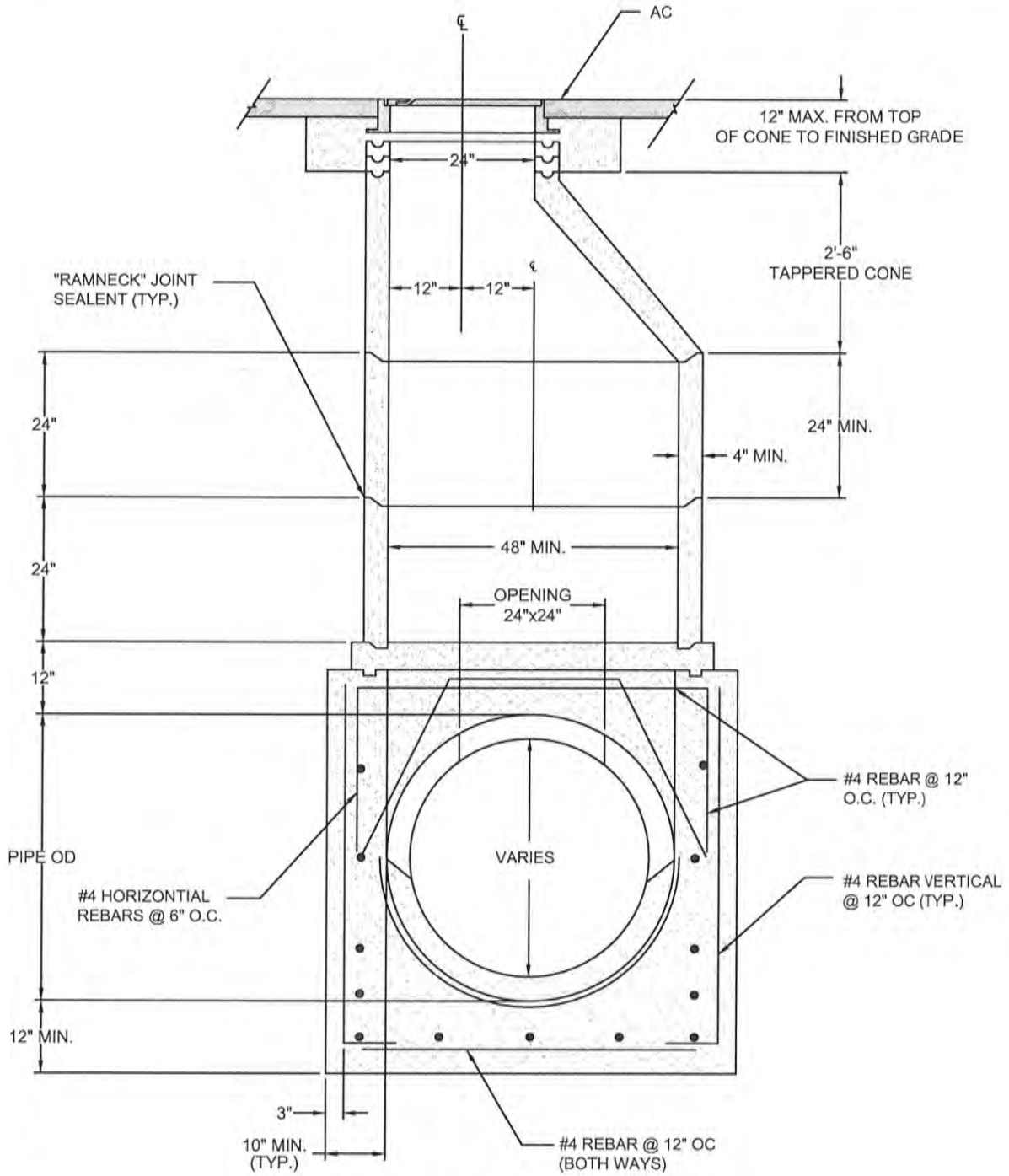
TYPICAL SECTION A-A
