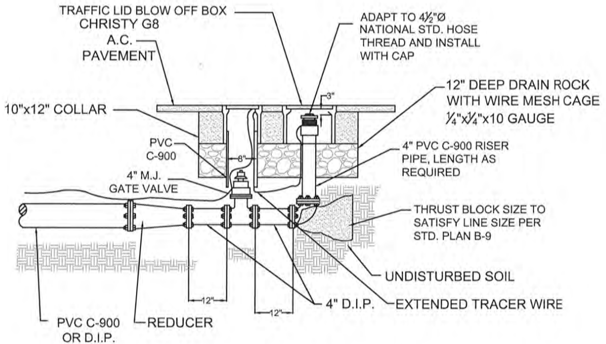
FOR 10" DIA. AND LARGER WATER MAIN
