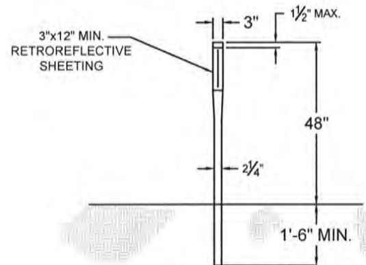
FLEXIBLE POST
