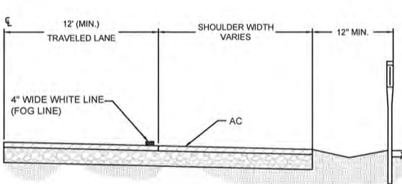
DELINEATOR POSITION
