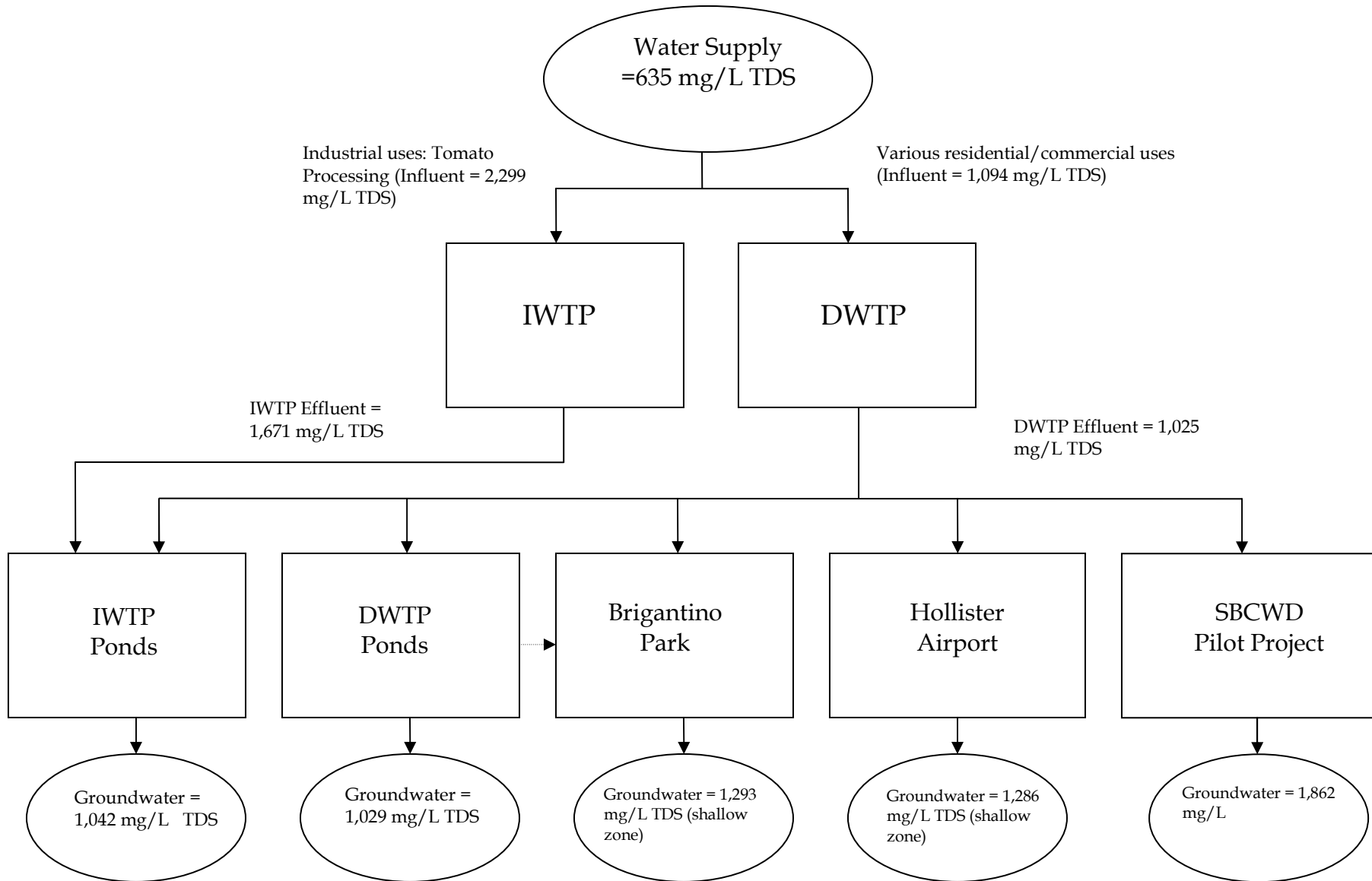
Figure 9. Salinity Pools and Transfers Associated with the DWTP and IWTP in 2010
