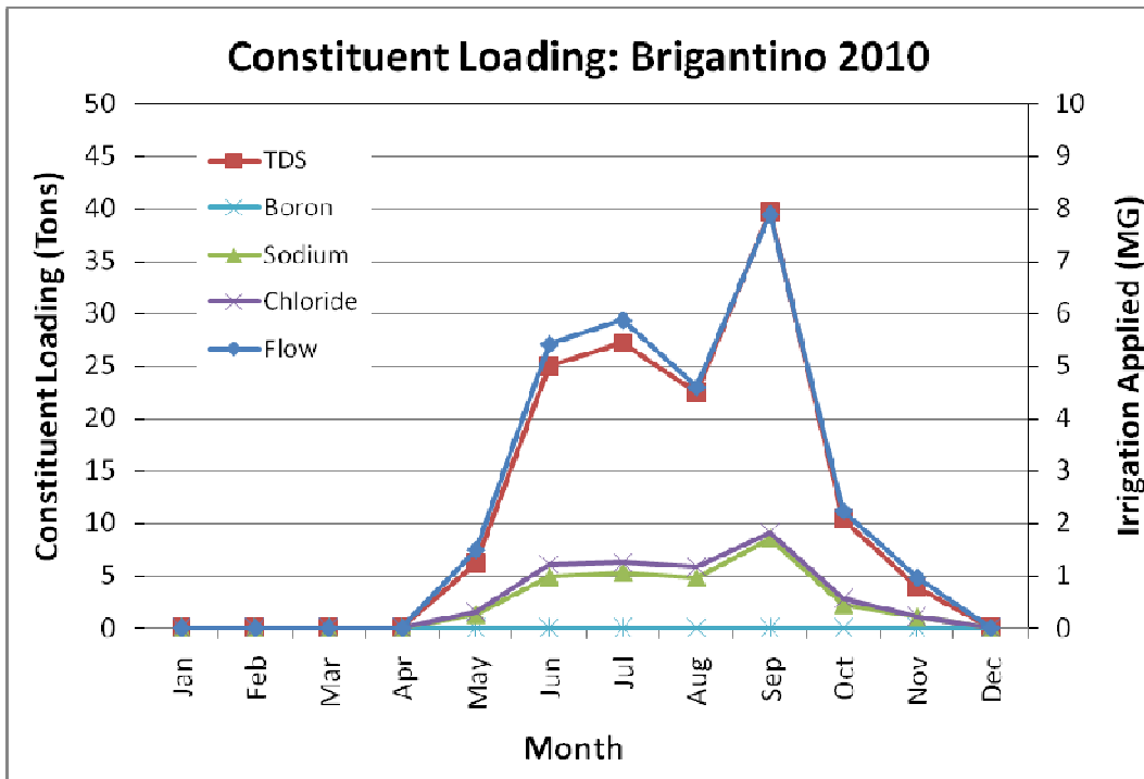
Figure 7.1. Monthly mass loading of selected constituents at Brigantino Park reuse area.
