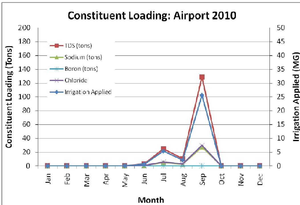
Figure 7.2. Monthly mass loading of selected constituents at Airport reuse area.
