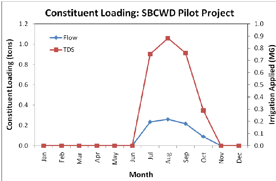
Figure 7.3. Monthly mass loading of selected constituents at SBCWD Pilot Project reuse area.
