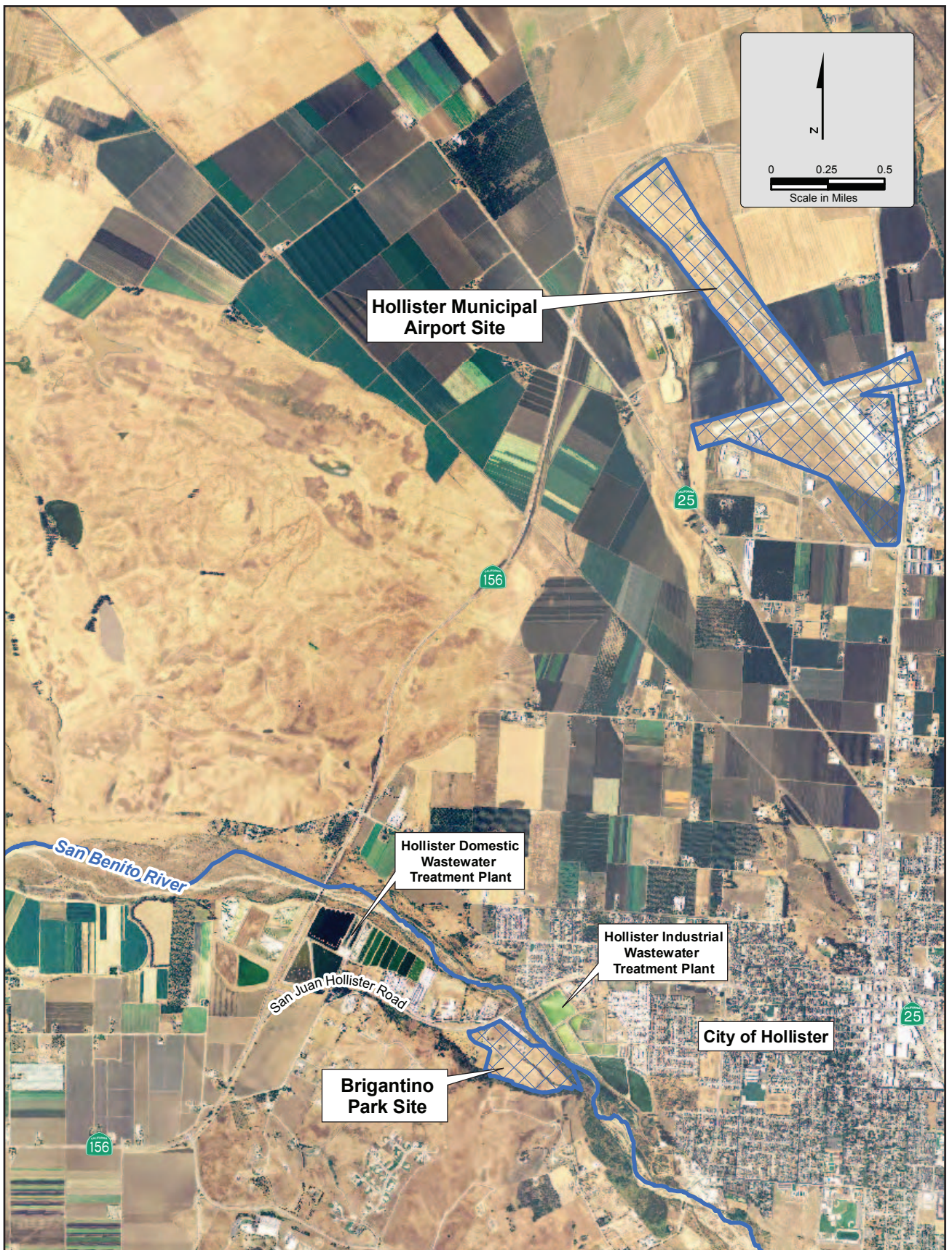
FIGURE 4 City of Hollister Recycled Water Use Areas
